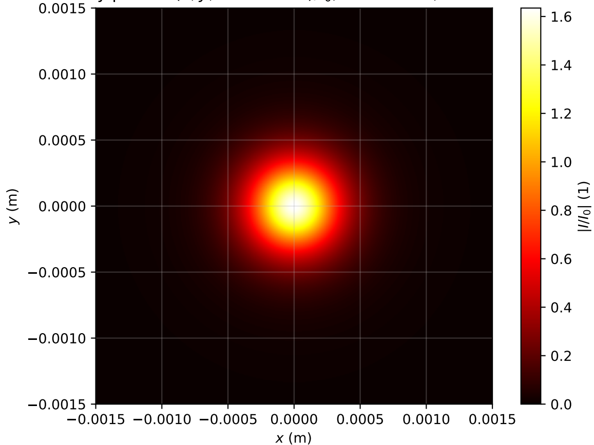
Intensity profile I(x, y, z = 2.149m)/I_0 , Pin=0.9Pcr, artificial time
